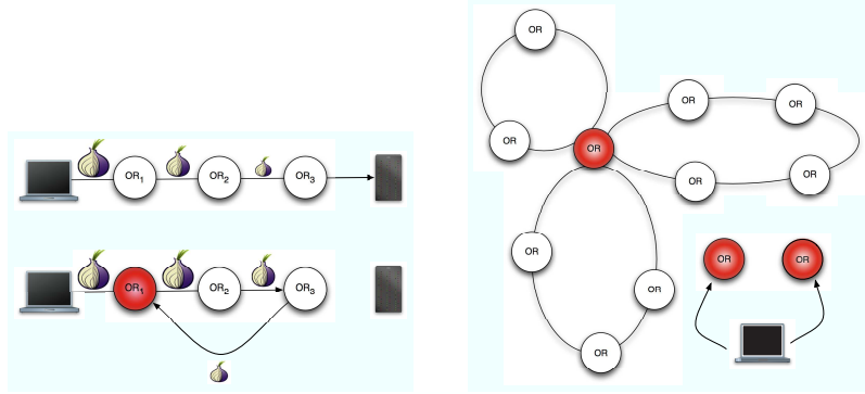
Fig. 1. Schematic representation of the packet spinning attack (LOOP phase). In the top part of the figure we depict the normal operation of a TOR circuit. Each OR decrypts a layer of the incoming packet and forwards it to the next one, until the packet reaches the final destination. In the lower part of the figure we depict the spinning attack. A malicious OR (solid cell), part of the circuit, injects again the initial packet in the circuit. The legitimate ORs continue to decrypt the packet in each spin, but the malicious one is not involved in any cryptographic operation.
