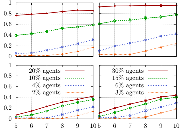
Fig. 6. Agents and users all start at trust level 6. Agents each recommend \{1,2\} new agents (left, right). Users \{are\ not, are\} grouped to servers by recommendation tree (top, bottom). Agent percentages refer to final fraction after recommendations.
